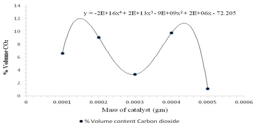
Fig. 2. Changes in the %composition of \text{CO}_2 gas from changes in the amount of catalyst in the reaction zone
